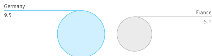
Carbon dioxide emissions in relation to France 2016 tonnes per capita
